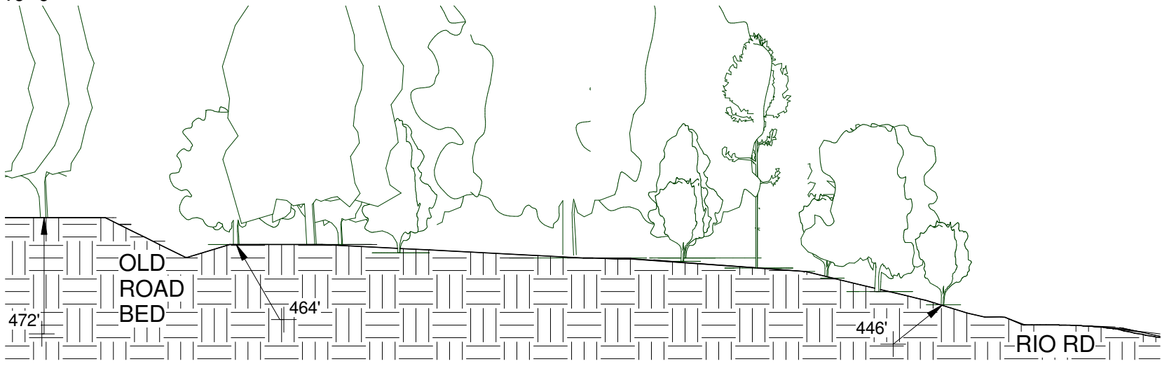
2 ROCKBROOK SECTION 2 1" = 40'-0"
